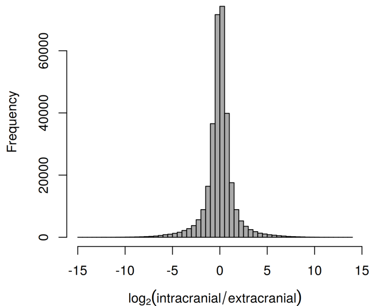
Figure S2: Histogram of gene expression \log_2 -ratios across all patient-matched intra- vs. extracranial melanoma metastases. The majority of genes has unchanged expression levels with values about zero. Down- and up-regulated genes in intracranial metastases have expression levels clearly different from zero.
