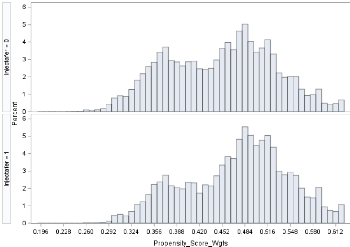
Distribution of Propensity_Score_Wgts
