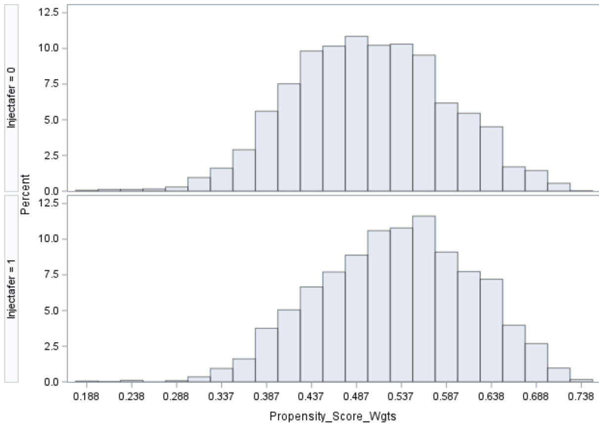
Distribution of Propensity_Score_Wgts
