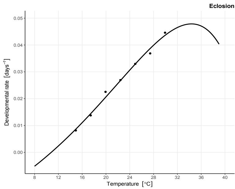
Fig. 1. Lactin-2 models fit to observed developmental rates of five development events of C. maxillosus . Black circles indicate observed data.
