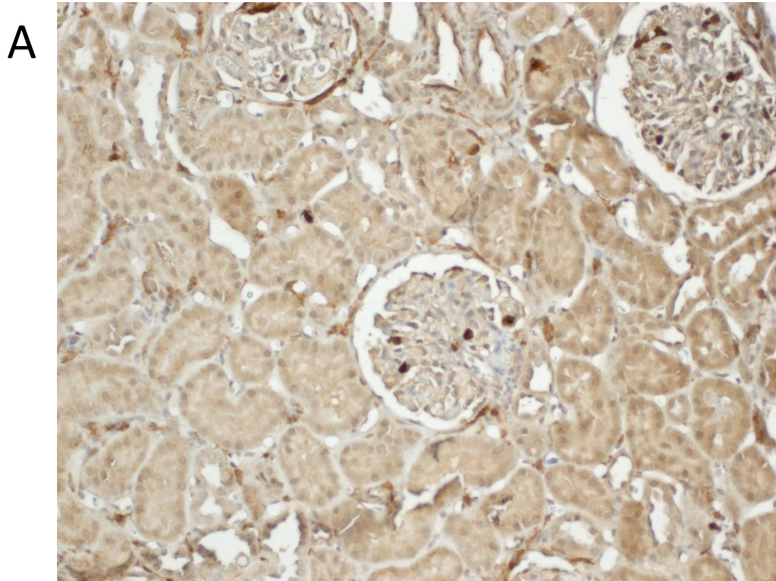
Expression of P-selectin glycoprotein ligand-1 in Henoch-Schönlein nephritis patient (A) and in control specimen (B)
