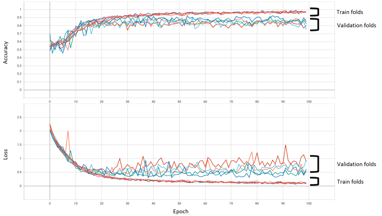
Figure S1: Training progresses of the 5 models generated during cross-validation.
